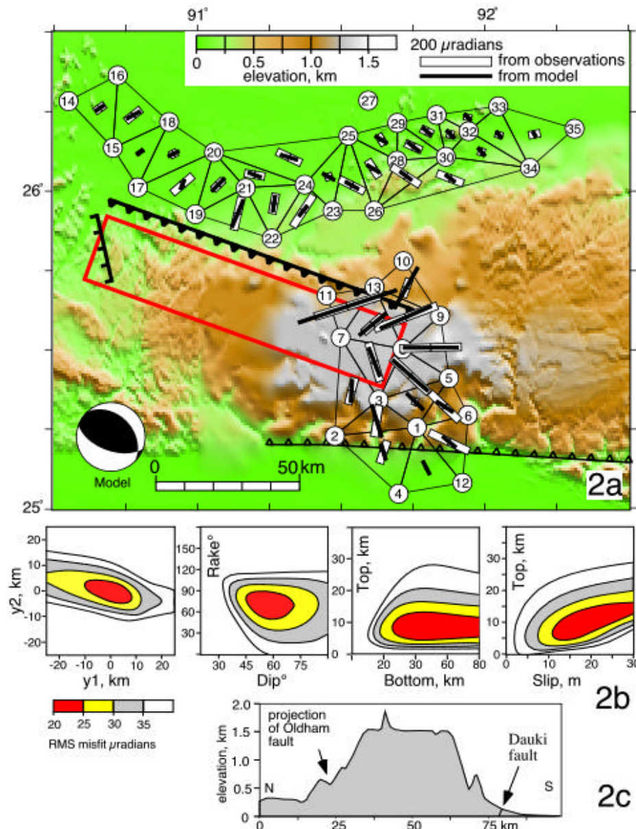
Figure 2a. Trigonometrical stations remeasured on 6 and north 9 of the Shillong Plateau following the 1897 earthquake. Shear strains for each triangle are displayed as bars whose orientations are parallel to the smallest (most compressional) principal strain and whose lengths are proportional to the shear strain, = \sqrt{\epsilon_1^2 + \epsilon_2^2} where \epsilon_1 = u/x - v/y , \epsilon_2 = u/y + v/x , and u, v are components of displacement in the easterly ( x ) and northerly ( y ) directions 11 . White rectangles are calculated from the triangulation observations, and black bars show the strains calculated for the best-fitting planar dislocation. Red rectangle indicates subsurface location of this SW dipping dislocation; thick black line with teeth shows the surface intersection of the continuation of this plane to the land surface (slip terminated 9 km below the surface). Short black line at western edge of fault plane indicates location of Chedrang fault, where Oldham 1 observed 11 m of co-seismic slip. Line with open teeth to south of the Plateau shows location of the Dauki fault. 2b Trade-offs between parameters of the model dislocation. Each panel displays the variation in root-mean-square misfit to the observed angular changes, with all parameters except those illustrated held fixed to their best-fitting values. y_1 and y_2 refer to latitudinal coordinate of, respectively, the western and eastern ends of the fault. 2c Topographic section through the central Shillong Plateau showing projected surface location of the Oldham fault. A peneplanation surface is evident at 1.6 km, with isolated peaks rising to 2 km.
