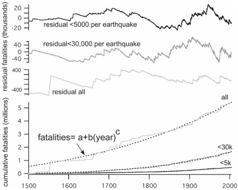
Fig. 12 Power law fits ( lowest graph ) and residuals to earthquake fatality data for the period 1500–1999. The parameters of these fits are listed in Table 2
