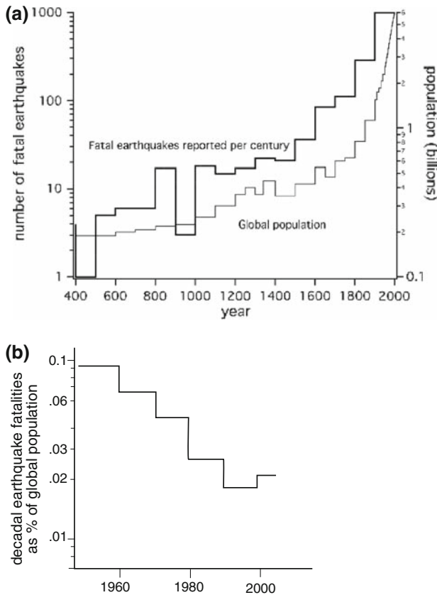
Fig. 6 a World population and numbers of fatal earthquakes per century increase steadily together. In this plot earthquakes are counted ignoring the numbers of fatalities in each earthquake (1 to >100,000). b The number of earthquake fatalities per decade normalized to the decadal global population averaged in five decade blocks. This view of earthquakes shows that earthquake risk to the individual averaged in a global sense has reduced in recent time
