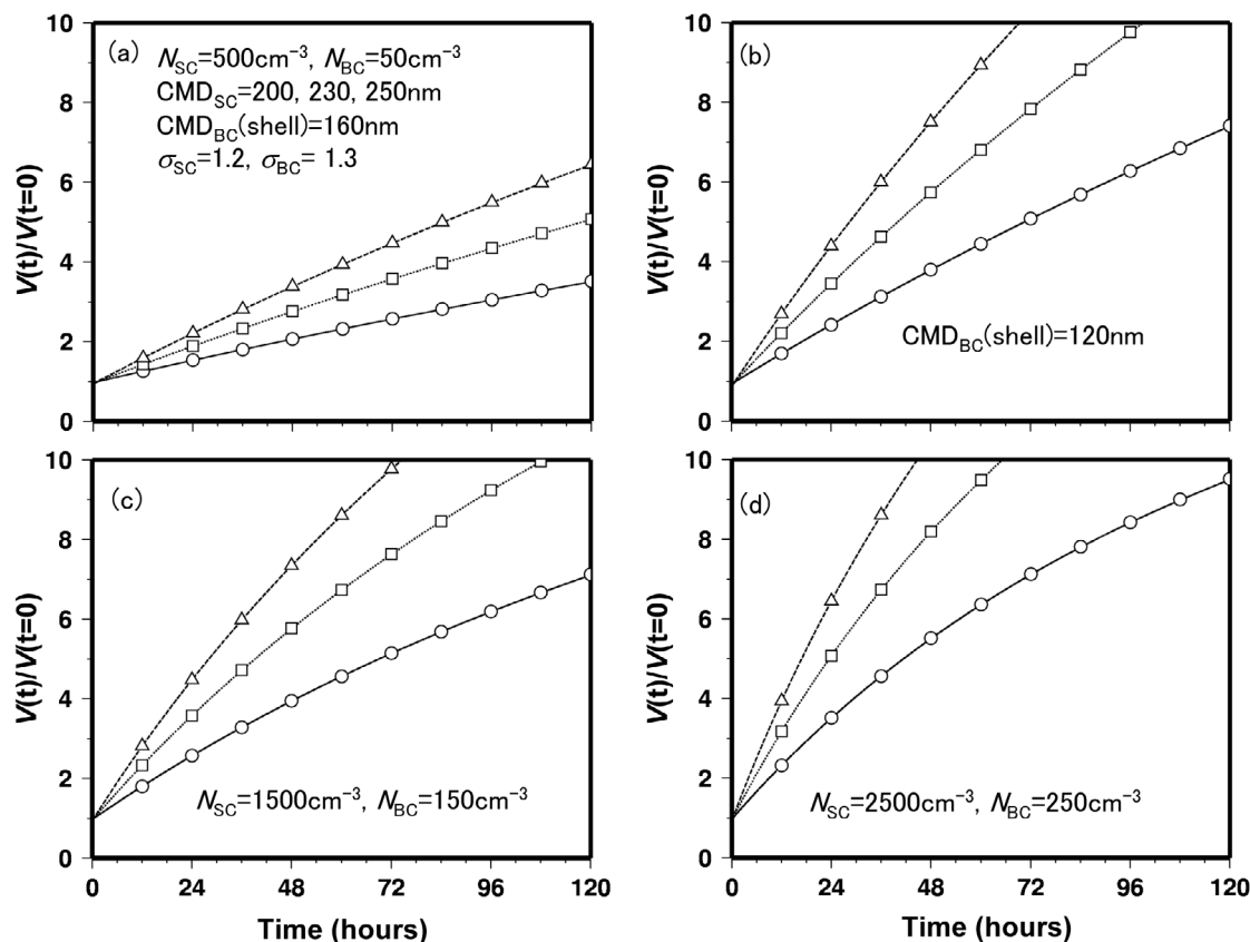
Figure 20. Time series of the ratios of the total shell volume of BC at time t ( V(t) = \int \pi [D_p(t)]^3 dD_p/6 ) to the initial V(t=0) shown together with the initial LNSD parameters. (a) Calculations for the conditions of CMD_{BC}(\text{shell}) = 160 nm. The lines with triangles, squares, and circles are the results for initial CMD_{LSP} = 250, 230 , and 200 nm, respectively. (b) Same as Figure 20a but for CMD_{BC}(\text{shell}) = 120 nm. (c and d) Same as Figure 20a but for initial N_{LSP} of 1500 and 2500 \text{cm}^{-3} , respectively.
