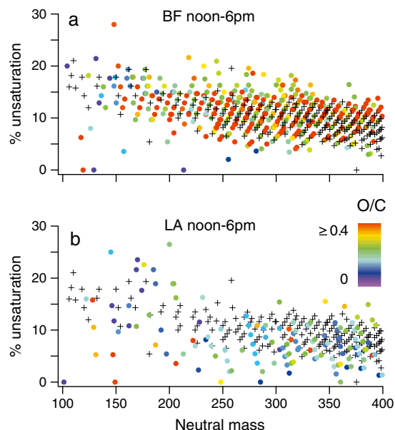
Figure 4. The percent unsaturation of each unique compound plotted vs. the neutral mass for (a) the BF noon to 6 P.M. sample and (b) the LA noon to 6 P.M. sample. The data are color-coded by the O/C value of the compound as indicated in the legend. The grey pluses are the common peaks for comparison.
