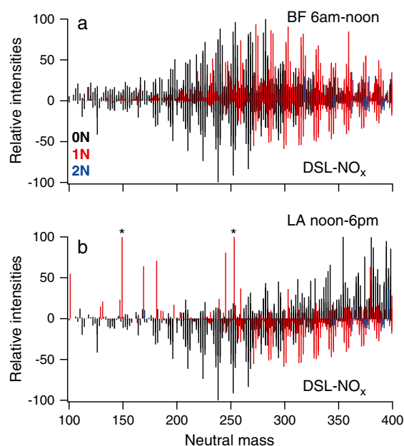
Figure 1. Comparison of the mass spectra of the ambient samples from each site with the best DSL- NO_x overlap: (a) BF 6 A.M. to noon and (b) LA noon to 6 P.M. The DSL- NO_x mass spectra are plotted with negative relative intensities to aid comparison. The colors correspond to the number of N atoms in the chemical formula with black = 0N, red = 1N, blue = 2N. The two starred peaks in the LA noon to 6 P.M. sample have intensities of 260 and 250 on this scale.
