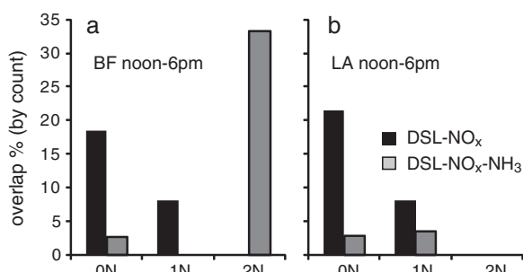
Figure 5. Percent overlap of the unique DSL-NO x and unique DSL-NO x -NH 3 peaks with (a) BF noon to 6 P.M. and (b) LA noon to 6 P.M. samples. The data are broken down by the number of nitrogen atoms in the chemical formula. The high overlap between 2N compounds and DSL-NO x -NH 3 peaks implies an important role of ammonia in forming nitrogen containing compounds in BF.
