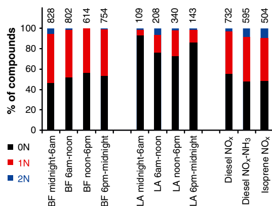
Figure 2. Percentage of formulas assigned 0N, 1N, and 2N for each sample. The 0N, 1N, and 2N compounds correspond to molecular formulas C c H h O o , C c H h O o N, and C c H h O o N 2 , respectively. The total number of identified peaks in each sample is shown above each column.
