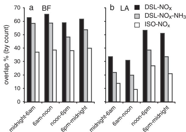
Figure 3. Percent overlap calculated from equation (1) for (a) BF and (b) LA samples with respect to the three chamber studies, DSL-NO x (black), DSL-NO x -NH 3 (gray), and ISO-NO x (white).
