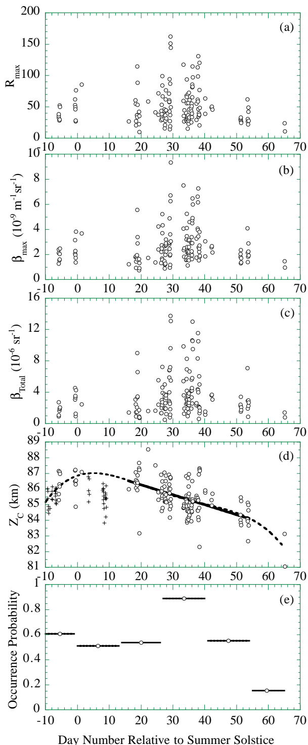
Figure 2. Seasonal variation of the hourly mean PMC (a) peak backscatter ratio, (b) peak volume backscatter coefficient, (c) total backscatter coefficient, (d) centroid altitude, and (e) PMC occurrence probability plotted versus day number relative to austral summer solstice (21 Dec 99). The open circles are the data from 374 nm lidar channel while the crosses are the data from 372 nm lidar channel. In Figure 2d, the dashed line is the 4 th order polynomial fit to all the 374 nm data, while the solid line is the linear fit to the 374 nm data between day 18 and day 53. The linear fit equation is Z_C(\text{km}) = 87.54 - 0.064 \text{ Day} , i.e., the slope is 64 m/day.
