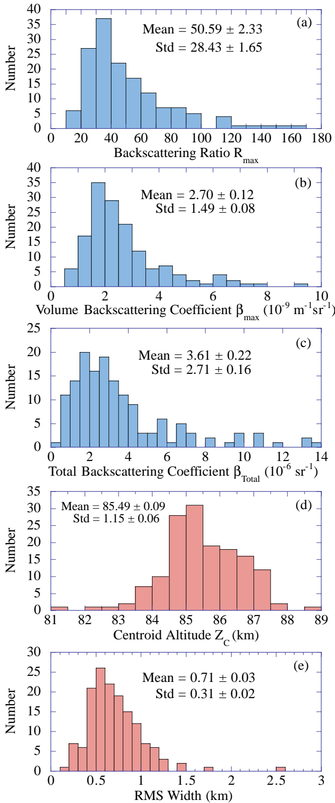
Figure 3. Histograms of PMC characteristics at South Pole in the 99-00 austral summer season derived from 149 h of 374 nm lidar data. (a) Peak backscatter ratio, (b) peak volume backscatter coefficient, (c) total backscatter coefficient, (d) layer centroid altitude, and (e) layer rms width.
