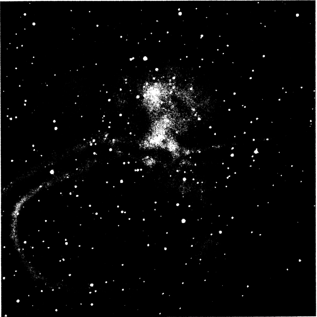
Plate 1. The Diamond Ring. Eighty two seconds after a -1.5 magnitude Leonid meteor appeared over Albuquerque at 0228 LT on November 17, 1998, its trail has been contorted into the appearance of a Diamond Ring. The 1 W sodium laser is the straight streak coming in from the right. The 502 pixel field of view is 1.94^\circ in this image, taken at an azimuth of 128^\circ and an elevation angle of 51^\circ . The scale of the image is obtained from the field of view and the known (from the lidar) mean slant range of 122.6 km.
