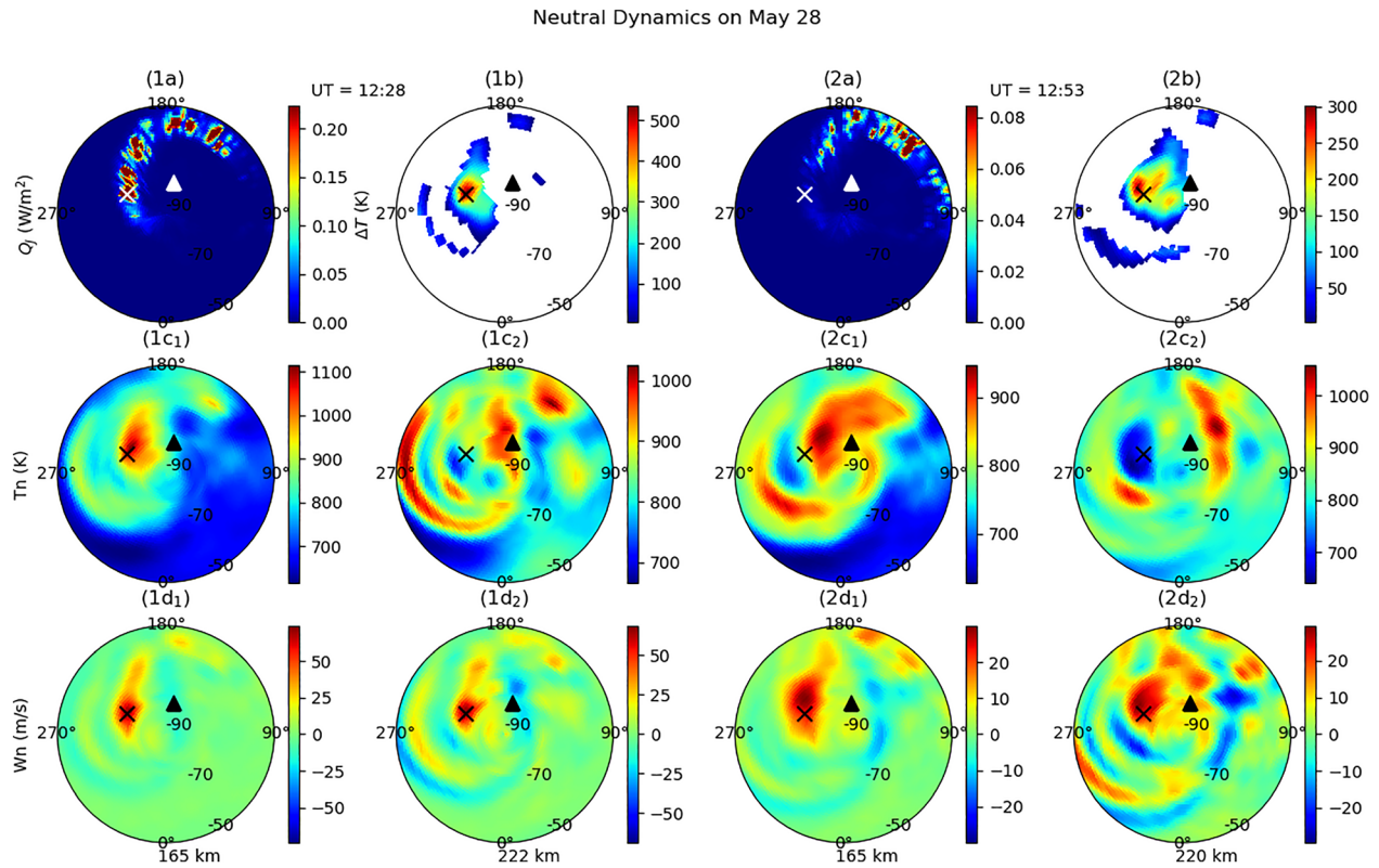
Figure 8. Spatial distribution of (1a) height integrated Joule heating, (1b) TTEIL magnitude, neutral temperatures at (1c 1 ) 165 and (1c 2 ) 222 km, and vertical winds at (1d 1 ) 165 and (1d 2 ) 222 km, at 12:28 UT in geographic coordinates. The 180° longitude is plotted at the top for a better visualization of the TTEIL propagation (see the movie provided in SI). The right two columns are the same except for 12:53 UT and the two examined altitudes are 165 and 220 km. Cross and triangle represent the location of the strongest TTEIL (73.75°S, 117.5°W) and McMurdo (77.8°S, 166.7°E), respectively.
