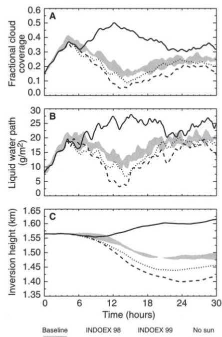
Fig. 4. Evolution of domain averages of (A) fractional cloud coverage (as defined in Fig. 3), (B) liquid water path (column of cloud water, in units of \text{g}/\text{m}^2 ), and (C) altitude of the trade inversion (mean height of the 6.5 g/kg total water mixing ratio surface, in km). Note that the liquid water path in (B) is averaged over clear and cloudy air; the average liquid water path in cloudy columns is greater by a factor inverse of the fractional cloud coverage in (A). Results are shown as centered 6-hour running averages to smooth over the convective noise seen in Fig. 2. Cloud droplet concentrations are fixed at 250 \text{cm}^{-3} for the simulations shown. For the baseline (gray area) the haze is nonabsorbing and the concentration is 1200 \text{cm}^{-3} ; for the INDOEX 1998 and 1999 cases (dotted and dashed lines), the haze absorbs solar radiation (as described in the text) and the concentrations are 1200 and 2400 \text{cm}^{-3} , respectively. For the modified baseline (solid line), solar radiation is omitted. For the baseline, an ensemble of four simulations was run (26); the gray area represents the range of values (after applying running averages) realized in the ensemble.
