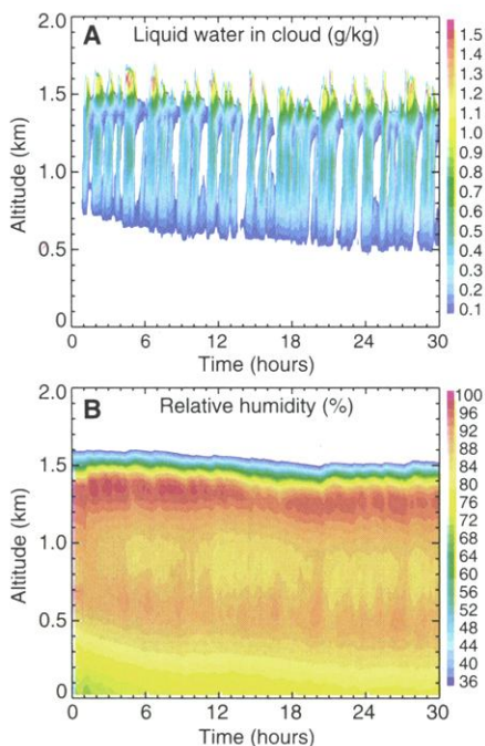
Fig. 2. Evolution of horizontal averages of (A) liquid water mixing ratio in cloud (grid cells with >0.05 g/kg liquid water) and (B) relative humidity in a baseline simulation. The profiles are output every 5 min.
