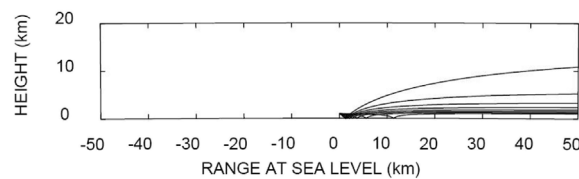
Fig. 14. Small extraordinary ray, downwind, f = 0.00125 Hz. Elevation angle of transmission varies from 50° through 85° in steps of 5°. Rays for elevation angles of transmission of 10° through 45° and 90° were evanescent at the source. The 50° elevation angle of transmission had rays that got the highest and had a pulse travel time of 88 h. The 55° elevation angle of transmission had a pulse travel time of 233 h. The source height is 1 km. Otherwise, conditions as in Fig. 12.
