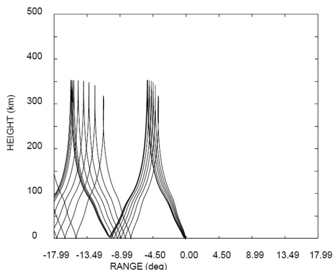
Fig. 13. Ordinary ray, upwind, f = 0.00125 Hz. The source is at a height of 5 km. The elevation angle of transmission is stepped from 10° degrees to 90° in steps of 5°, but waves for elevation angles of transmission of 55° and higher are evanescent. Otherwise, conditions as in Fig. 12. The 10° elevation-angle ray reaches an apogee of 353 km at a range of 589 km in 2 h. The 50° elevation-angle ray reaches an apogee of 318 km at a range of 422 km in 3.6 h.
