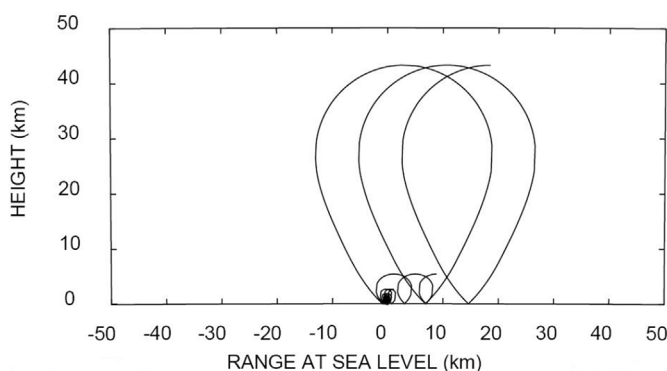
Fig. 15. Small extraordinary ray, upwind, f = 0.00125 Hz. Elevation angle of transmission varies from 10° through 45° in steps of 5°. Rays for elevation angles of 50° through 90° were evanescent at the source. Rays for 45° elevation angles reached the highest and had a pulse travel time of 62 h to the apogee and a total of 122 h from the source back down to the first ground reflection. Rays for 40° elevation angles reached a height of 5.4 km with a pulse travel time of 50 h and a total of 93 h from the source back down to the first ground reflection. Otherwise, conditions as in Fig. 14.
