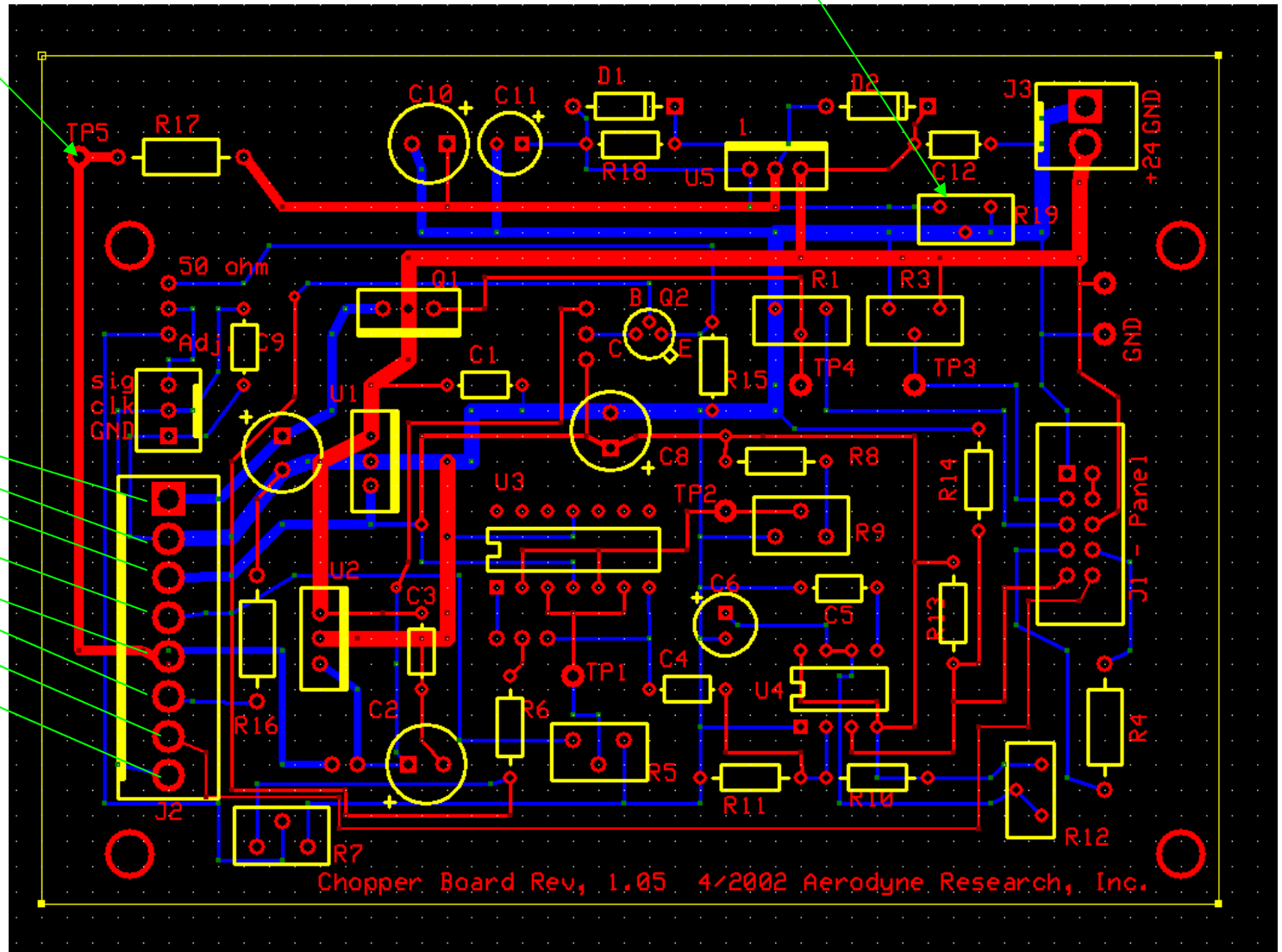
Chopper circuit board inside the AMS Electronics Box
