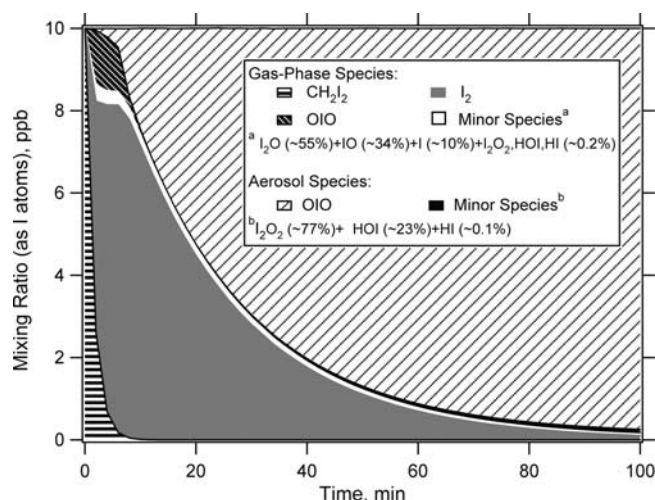
Figure 13. Simulated concentration profiles of the main iodine species for the simulation base case S1 (5 ppb CH 2 I 2 , 100 ppb O 3 , 2% RH), which corresponds to the conditions of the experimental base case E1. This is a stacked plot: the vertical extent of each band represents the mixing ratio of each species (as iodine atoms) at a given time, and the total number of iodine atoms in the system remain constant. Concentrations of the species not in the legend are too small to be seen in the graph.
