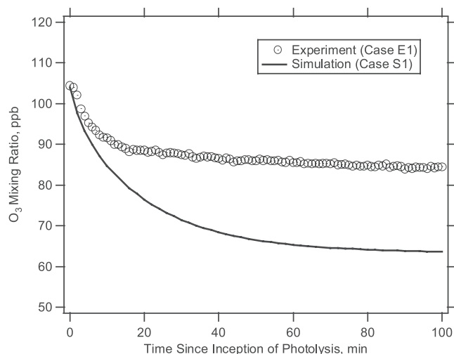
Figure 15. Comparison of the observed and predicted O_3 concentrations evolutions as a function of time since inception of photolysis for the base case (cases E1 and S1).
