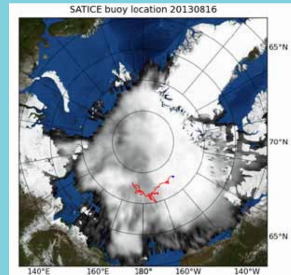
The motion of one of the SATICE buoys from August 2012 until August 2013. Courtesy of P. Elosegui, M. Olsson, SATICE Project
