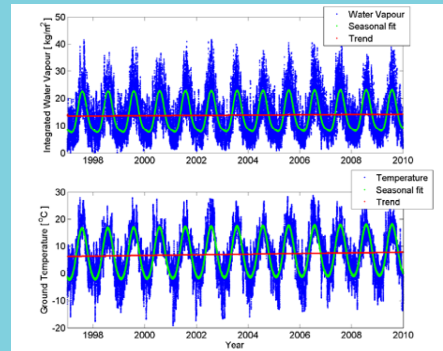
The water vapour content and the temperature at the ground for 14 years at the GNSS site Onsala in Sweden. The blue dots are hourly observations. Modelling a linear trend (red lines) and seasonal components (green lines) gives a trend for the water vapour content and the temperature of 0.5 kg/m²/decade and 1.1 °C/decade, respectively.
