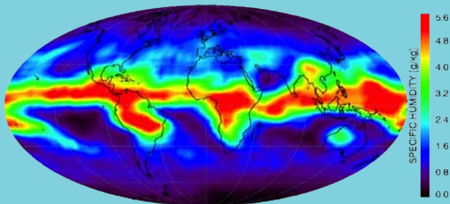
Monthly mean for October 2006 of the global distribution of specific humidity at the 600 hPa pressure level, at an altitude of about five kilometres. Derived from GNSS radio occultation measurements. Courtesy of S. Heise, GFZ
