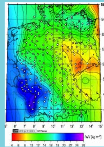
The water vapour content over Germany derived from ground-based GNSS stations. Courtesy of G. Dick, GFZ
