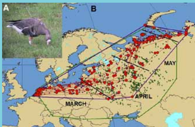
Recordings of white fronted goose in 2006–2008. Red dots represent GNSS positions, while green dots represent additional metal ring recordings. Courtesy of www.blessgans.de
