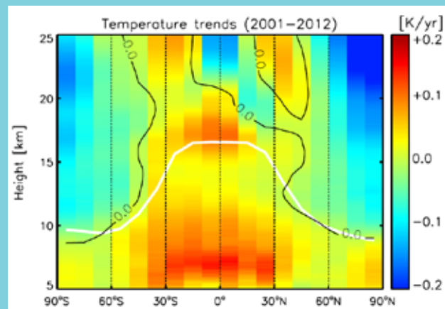
Temperature trends in the upper troposphere and lower stratosphere (5–25 km) derived for the period 2001–2012. The resolution in height and latitude is 100 metres and 10°, respectively. The solid white line denotes the mean tropopause height.
