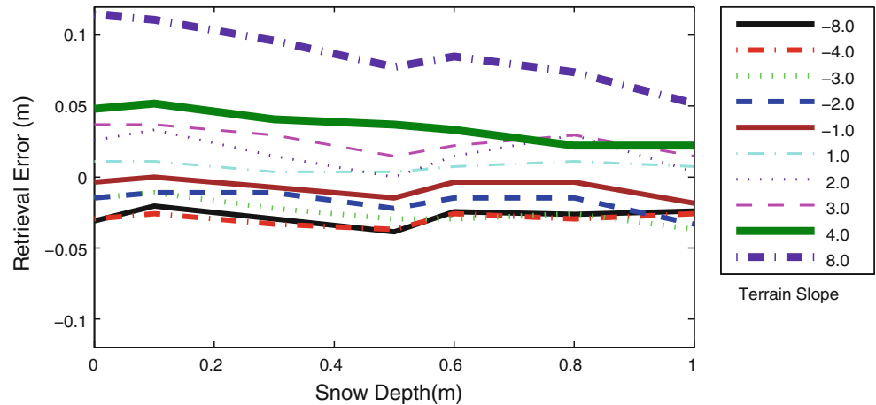
Fig. 5 Effect of terrain slopes (degrees) on snow depth retrievals
