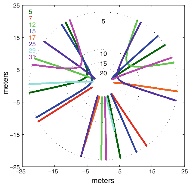
Fig. 3 Multipath reflection points for L2C satellites recorded at PBO site p360 on July 19, 2011
