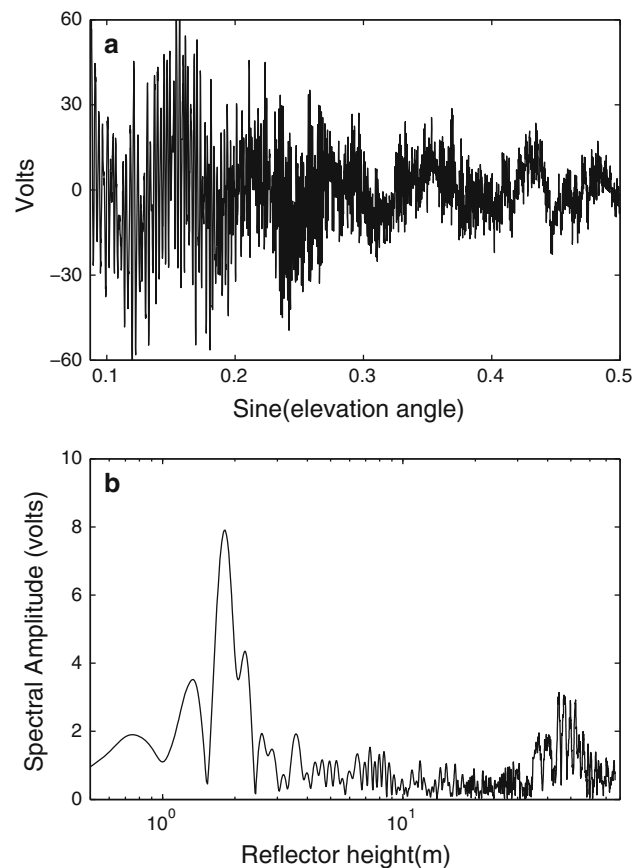
Fig. 9 Top GPS SNR data for PRN 31 in NE quadrant at PBO station p101; bottom Lomb-Scargle periodogram of data in top panel
