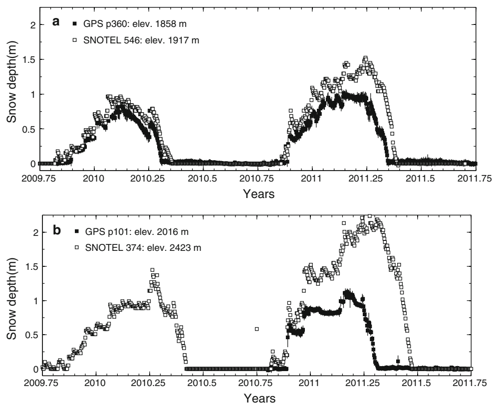
Fig. 10 GPS snow depth retrievals from PBO sites p360 and p101. Standard deviations represent the standard deviation of the individual satellite tracks and a formal error of 2.5 cm, added in quadrature. SNOTEL data are also shown
