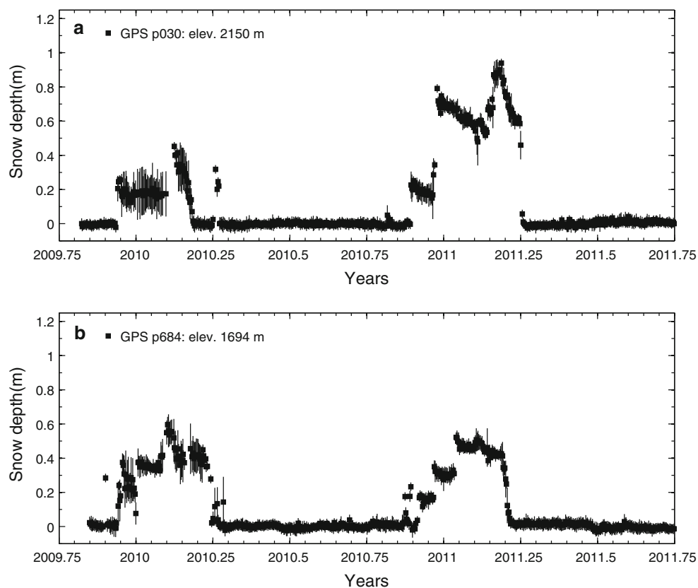
Fig. 11 GPS snow depth retrievals from PBO sites p030 and p684. Standard deviations represent the standard deviation of the individual satellite tracks and a formal error of 2.5 cm, added in quadrature
