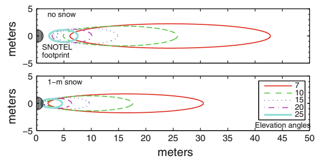
Fig. 4 First Fresnel zones for a satellite rising from the east are depicted for elevation angles from 7 to 25^\circ . Antenna height is set at 2 m for both figures. In the top panel , no snow is present. In the lower panel , the Fresnel zone is computed for a meter of snow. The snow-sensing zone for each GPS site could in principle include one of these Fresnel zones for each ground tracks shown in Fig. 3. Half of the SNOTEL footprint is shown centered at zero
