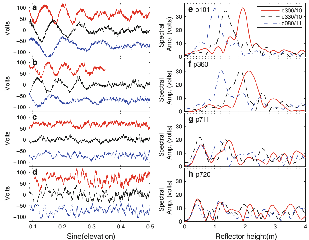
Fig. 6 a–d SNR data for representative tracks at sites p101, p360, p711, and p720. Day of year 300 (2010) represents bare soil reflections; day of year 330 (2010) and 80 (2011) represent days with low and high snow levels. Lomb-Scargle periodograms computed for the SNR data are shown in the right panels in plots (e–h)
