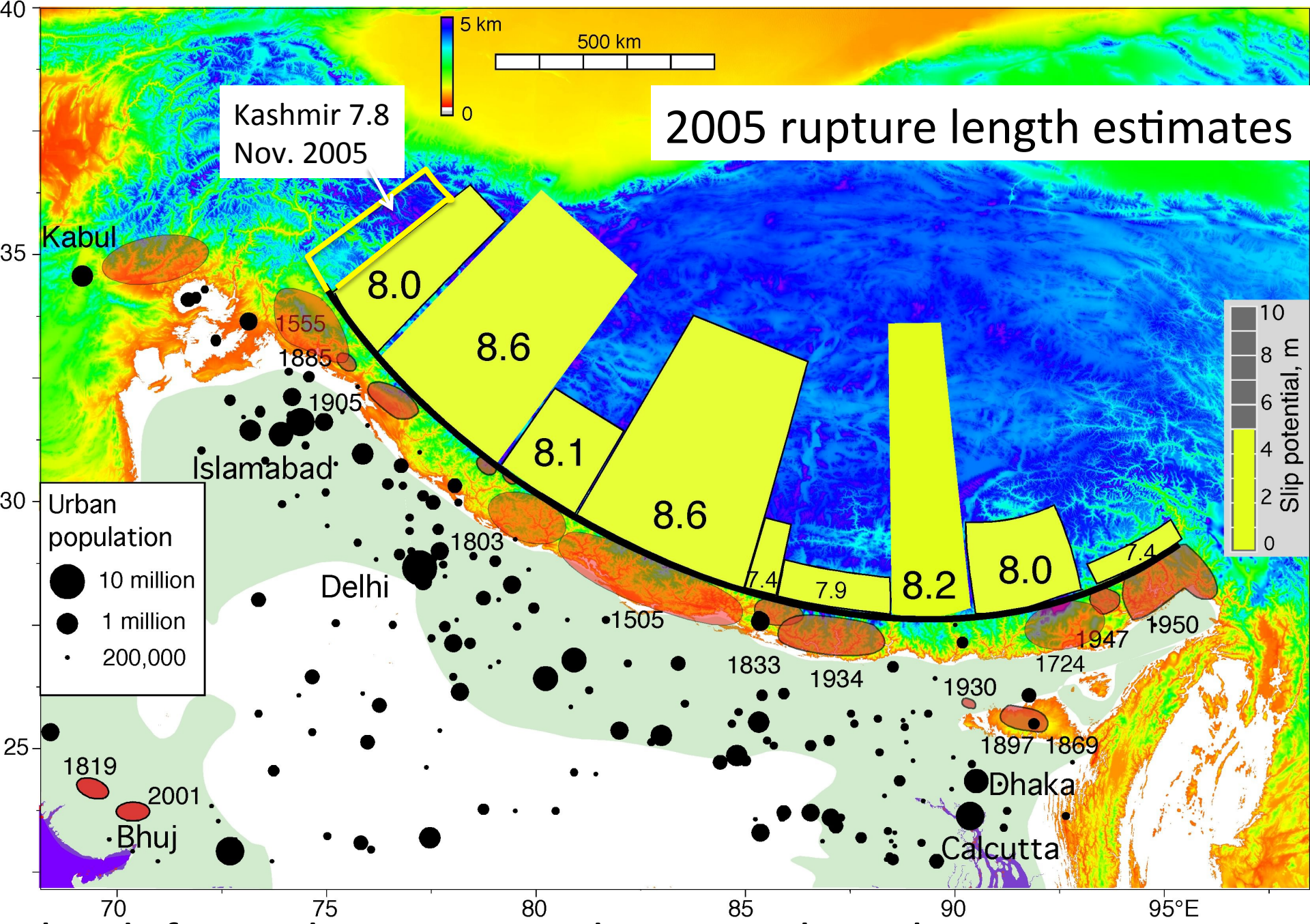
slip deficits plus estimated rupture lengths
