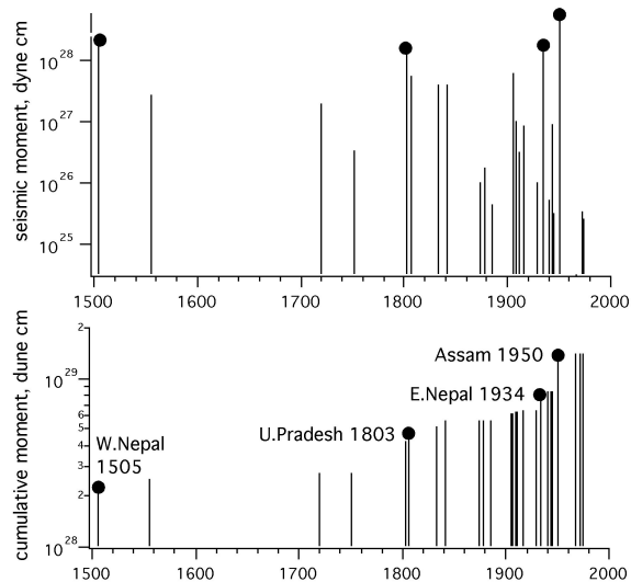
Fig.2 The release of seismic moment with time shows that we are probably missing numerous earthquakes in historical seismic record, especially in the 16 th and 17 th centuries. The large 1713 earthquake in Bhutan (ref.3), for example, cannot yet be assigned a magnitude. It is also clear that most of the moment release occurs during the largest earthquakes ( M > 8 indicated by dark circles).
